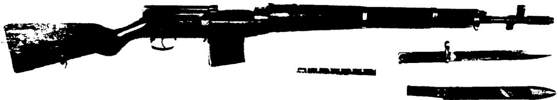
FIGURE 53. 7.62-MM SEMIAUTOMATIC RIFLE M1938 (SVT).
